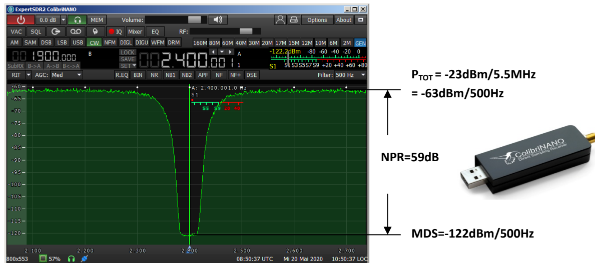
Figure 6: ColibriNANO with B_{RF}=5.5\text{MHz} , NPR = 59dB
