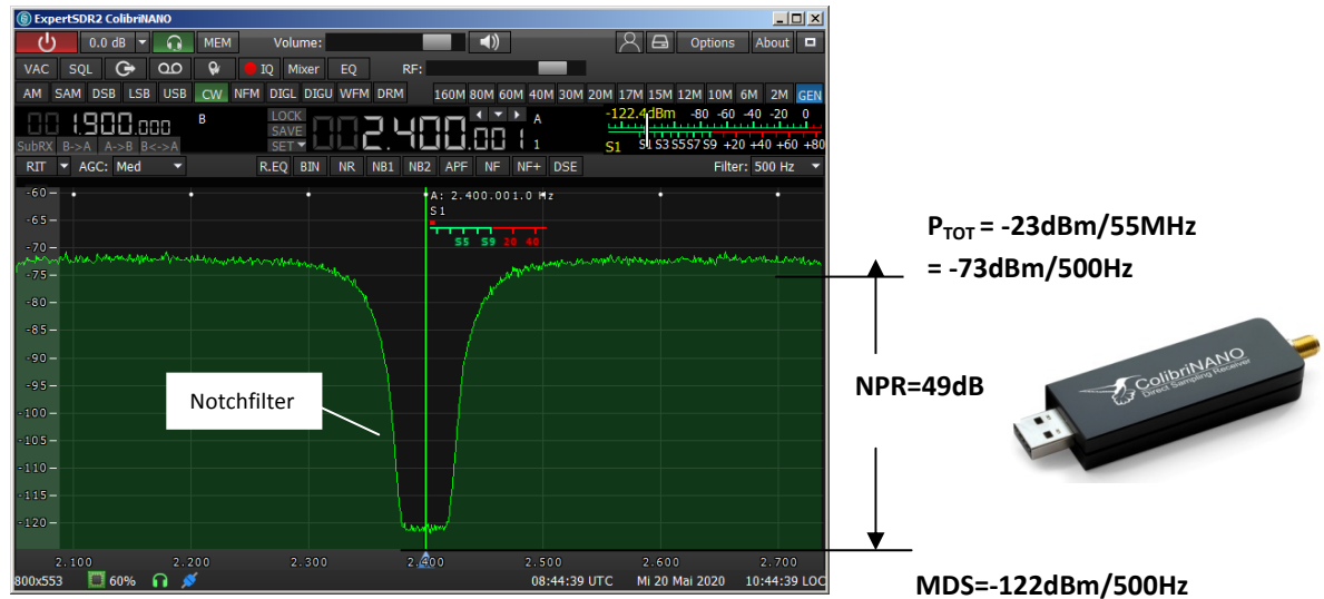
Figure 5: ColibriNANO with B_{RF}=55\text{MHz} , NPR = 49dB
