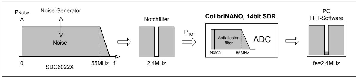
Figure 4: NPR measurement at ColibriNANO
