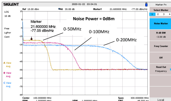
Figure 3: Noise signals of the SDG6022X
