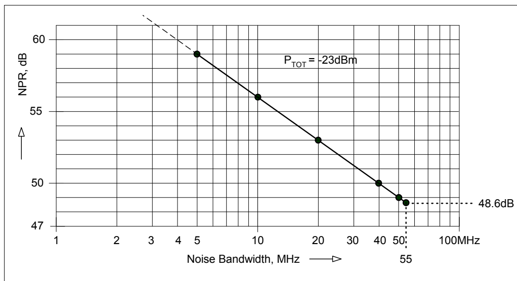
Figure 7: NPR of the ColibriNANO as a function of the injected noise bandwidth
