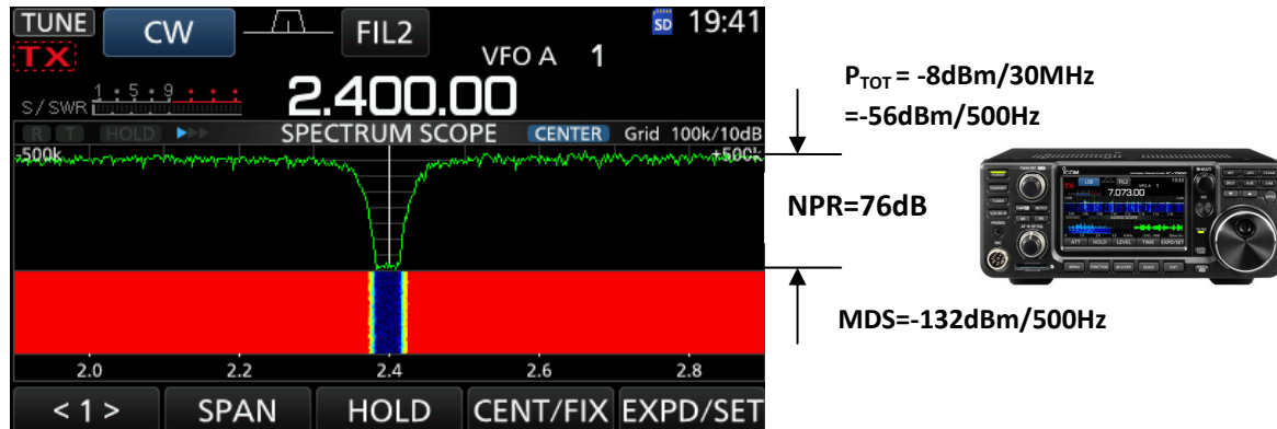
Figure 9: IC-7300, NPR = 76dB
