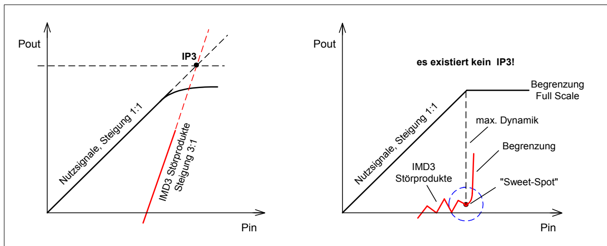
Figure 1: Principle IMD3 curve of an analogue receiver (left) and digital receiver (right)
