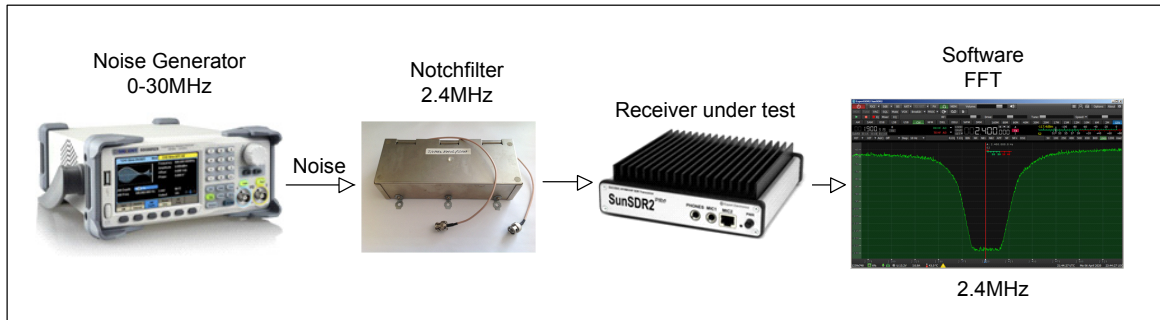
Figure 2: NPR measuring station
