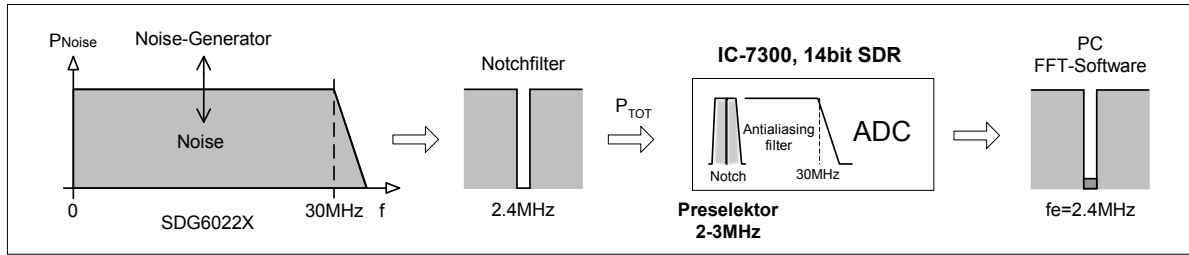
Figure 8: NPR measurement on the IC-7300
